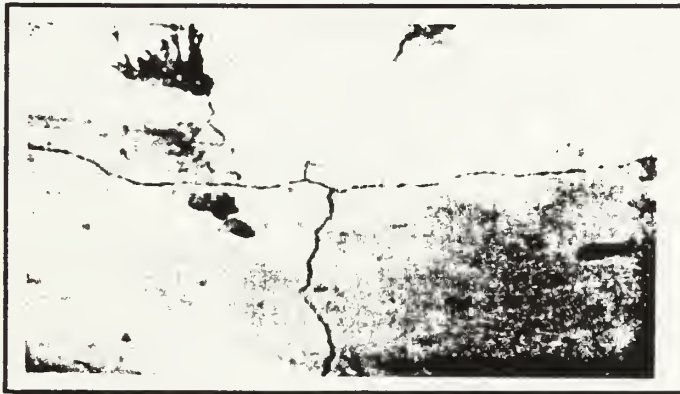
Figure 2.8 Typical drying shrinkage cracks (Reference 3)
